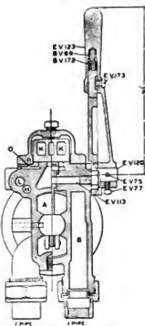
Fig. 2578. Cross-Section Through Main Slide Valve.
